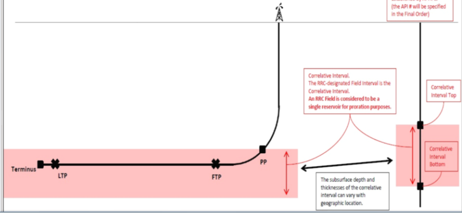
FIELD RULE ILLUSTRATION: WELLBORE SIDE VIEW OF WELL #1 ABOVE
